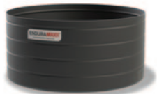
15,000 Litre 17204001 3450 dia x 1555 H 3299 gallons 15 cubic metres
